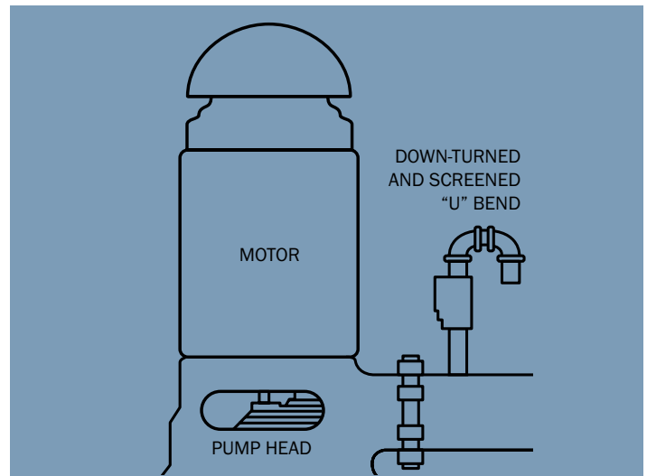
3 EXAMPLE “U” BEND. Air vents should be protected against the entrance of foreign material by installation of down-turned and screened “U” bends. Source: graphic recreated from DWR Bulletin 74-81 ( http://www.water.ca.gov/pubs/groundwater/water_well_standards_bulletin_74-81/ca_well_standards_bulletin74-81_1981.pdf ).
