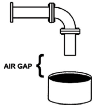
4 AIR GAP. An air gap is a vertical, physical separation between the end of a water supply outlet and the flood-level rim of a receiving vessel. An air gap is considered the maximum protection available against backpressure backflow. Source: American Backflow Prevention Association, http://www.abpa.org .
